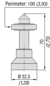
Adaptor-PPC-04/12-SKA-Contact
