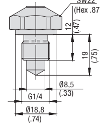
Screw-in Temperature Sensor (T) Process Connection M10x1 Process Connection G1/4 Rod-type Temperature Sensor (TSH)
