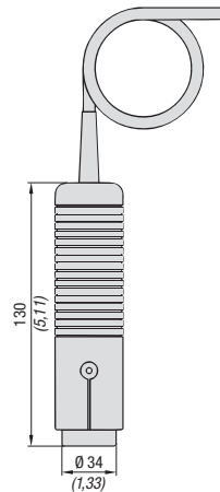
Sensor-PPC-04/12-SDS-CAB
